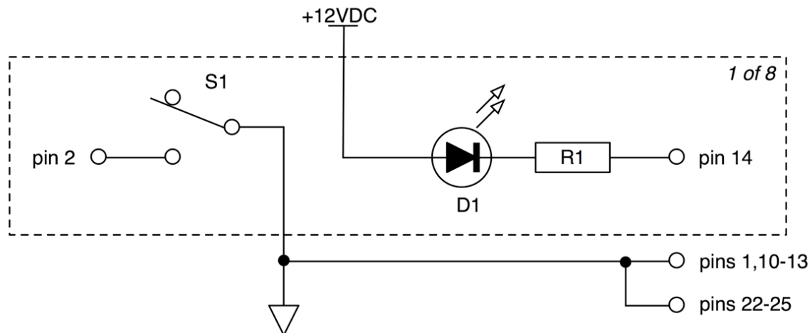
Figure E.1. GPIO Test Fixture Schematic
